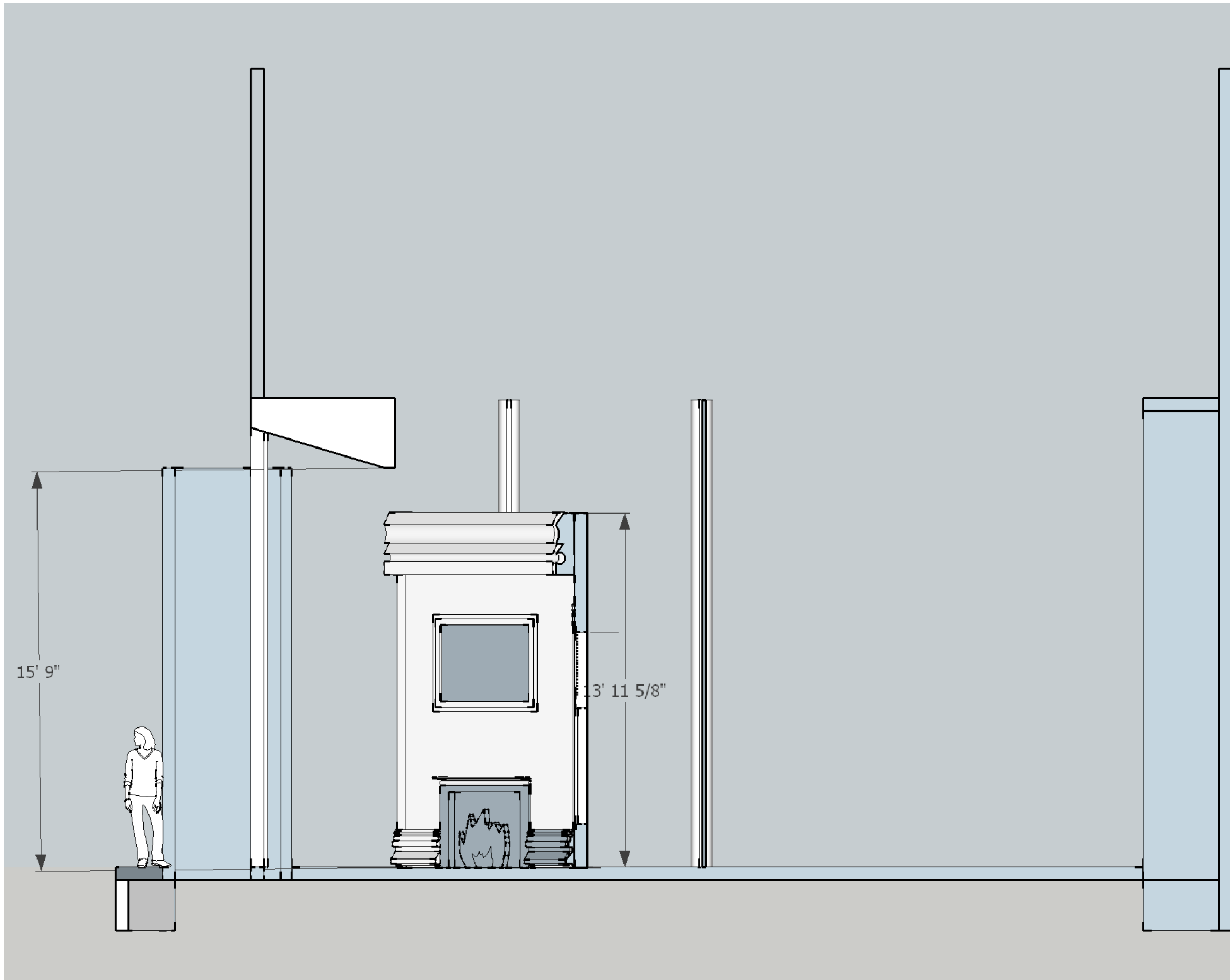
Man and Superman Centre Line Section Frederic Wood Theatre Scale: 1/4" = 1' - 0" Designer: Chengyan Boon Advisor: Robert Gardiner Date: 12/02/13
